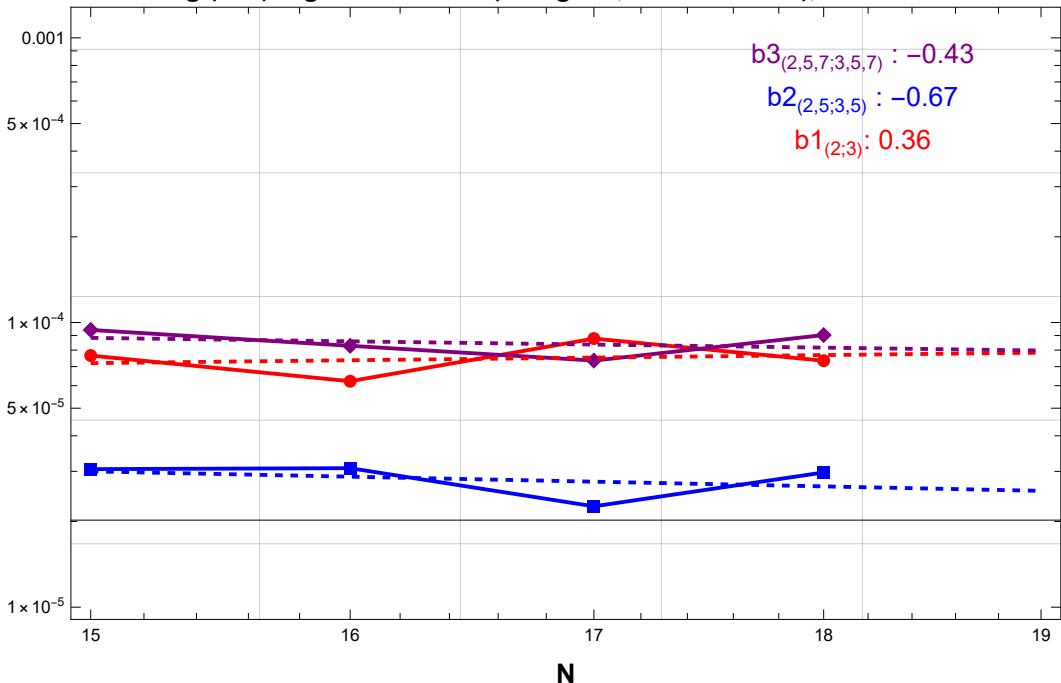
TAvg (0-2) Signal at Site 13 (Jlong=20; Jx = rescaled), \alpha=0.5 - Close
